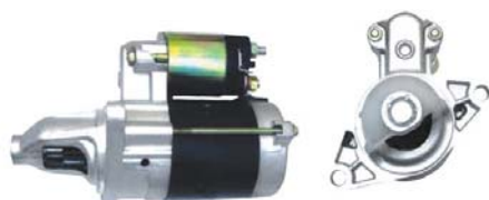
1015201GA00A 12V/1.4KW/8T/CW
