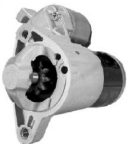
17939 12V/1.2KW/10T/CW MOT31471 JEEP LT TRK
