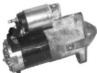
17882 12V/1.2KW/10T/CW MOT92081
