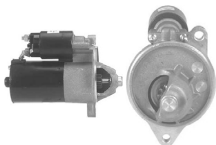
3235 2-1568-FD PMGR Ford 12V 1.5KW 10T
