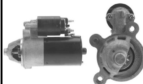
6654 2-1898-FD PMGR Ford 12V 12T
