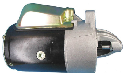
3212 2-1687-FD 4-1/2 in. MOD II Ford 12V 9T
