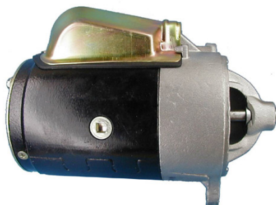
3176 2-1676-FD 4-1/2 in. MOD II Ford 12V 9T
