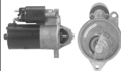
3234 2-1565-FD PMGR Ford 12V 1.5KW 10T
