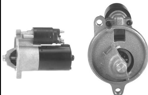
3240 2-1895-FD PMGR Ford 12V 1.4KW 10T
