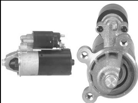
3269 2-1801-FD PMGR Ford 12V 1.4KW 10T
