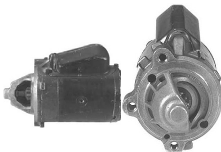
6657 2-2218-FD PMGR Ford 12V 1.5KW 11T
